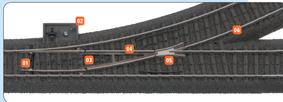
01 Separately mounted, cast switch rails 02 Prototypical built-up roadbed area at the location for the switch linkage 03 Continuous electrical contacts from the switch rails to the frog 04 Intermediate rails made of shaped material 05 Inset metal frog 16° 06 Turnout curve as a 24.3° section of a circle, radius 437.5 mm / 17-1/4"
